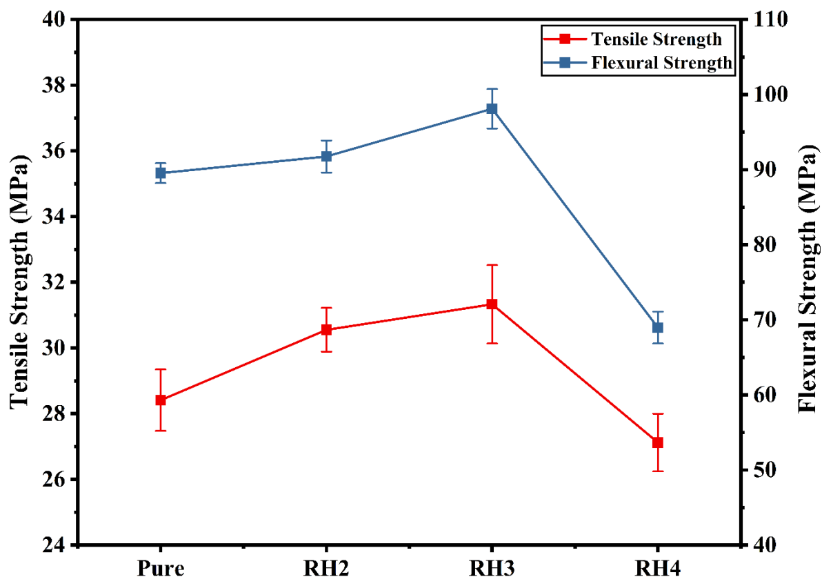
Figure 1. Tensile and flexural strength chart of reference and composite samples.
