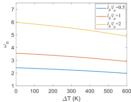
Figure 4. Examination of \omega_n with respect to l_b/l_a and \Delta T ( V_{\text{GPL}}=0.1 , p=1 ).
