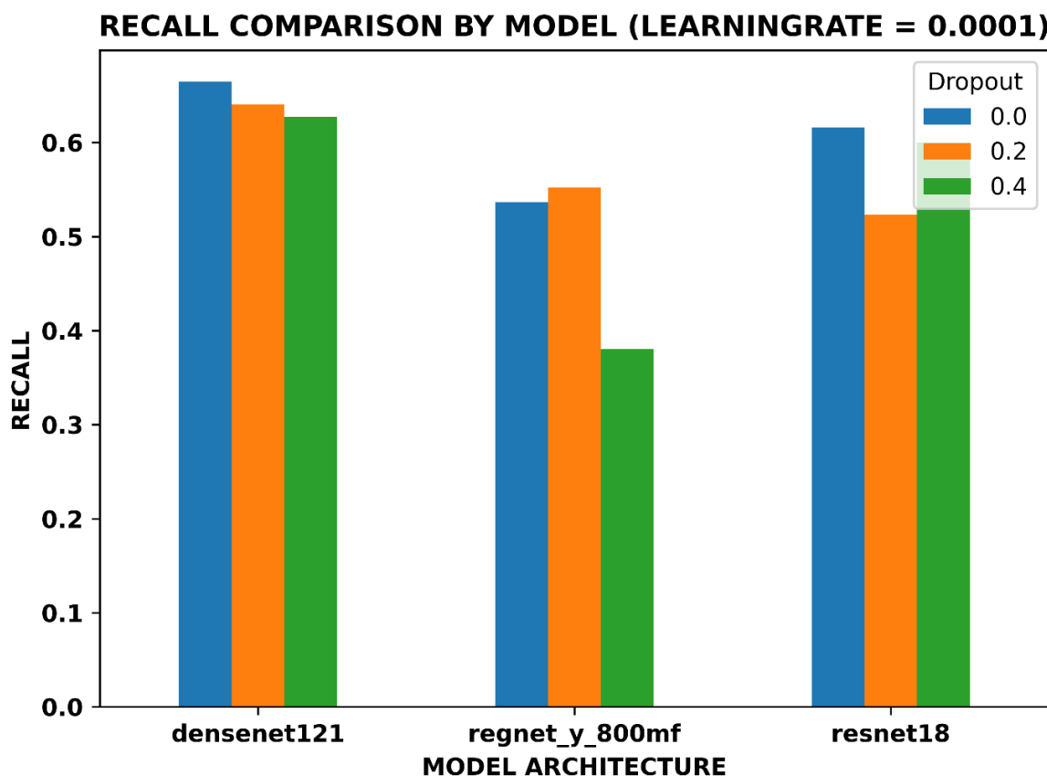
Figure 3 Recall Comparison by Model (Learning Rate = 0.0001)
