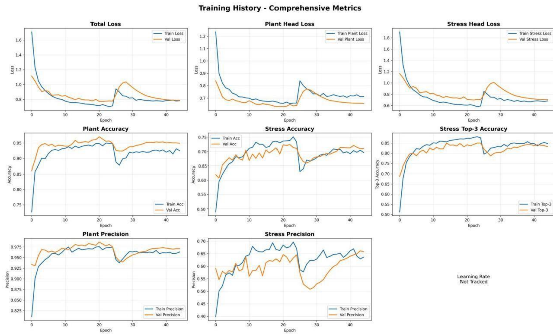
Figure 3. CNN Training History: Comprehensive Metrics
