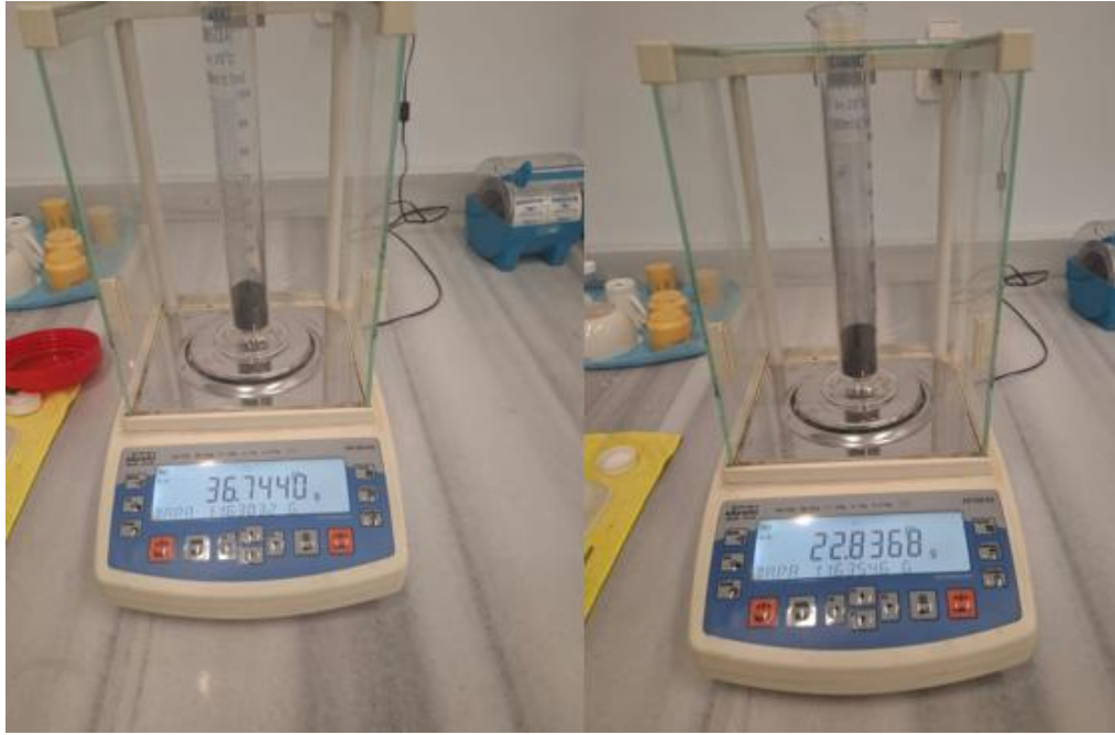
Figure 15. Chimney and iron dust masses.
