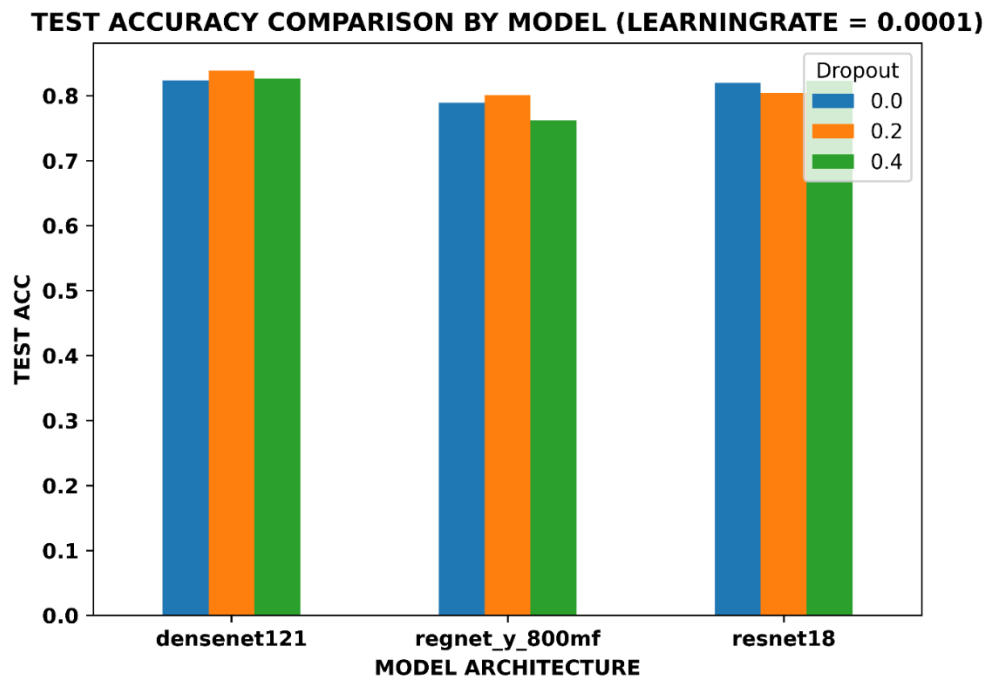
Figure 8 TEST ACCURACY COMPARISON BY MODEL (DROPOUT = 0.2)
