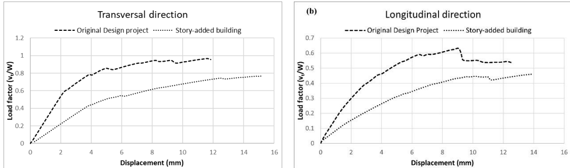
Figure 5. Capacity curves of the original project and story added building
