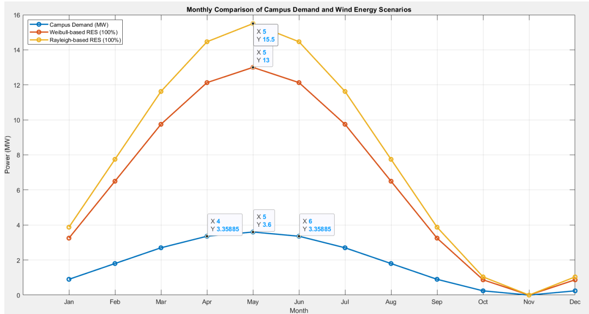
Figure 1. Monthly comparison of campus electricity demand derived from billing data with wind energy scenarios modeled using Weibull and Rayleigh distributions, illustrating the closer agreement of the Weibull model with the observed campus demand profile.
