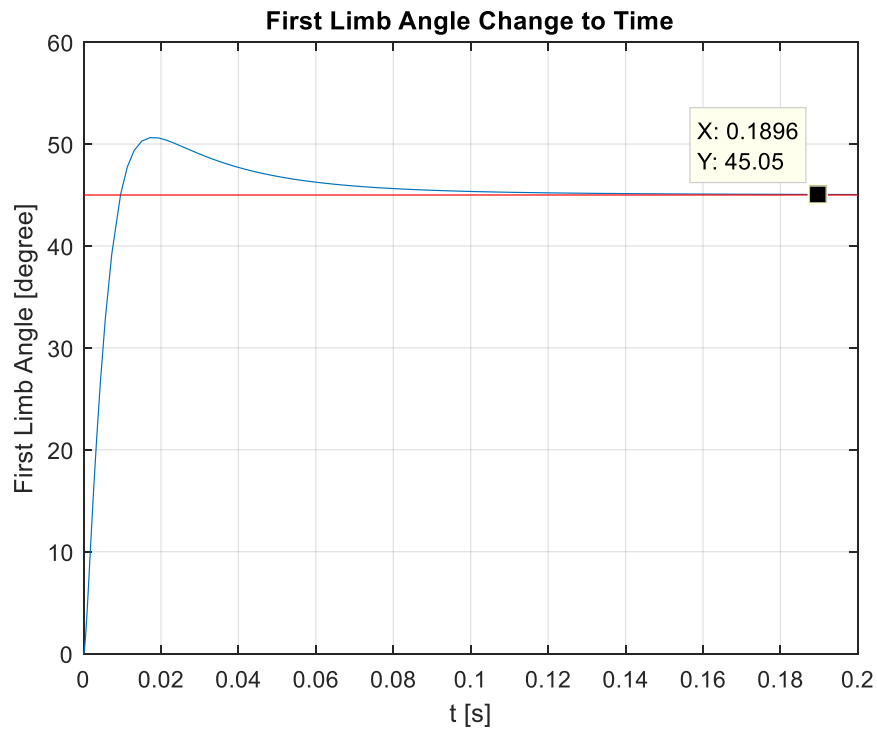
Figure 9. First Limb Angle Change to Time of Two-Loop Mechanism
