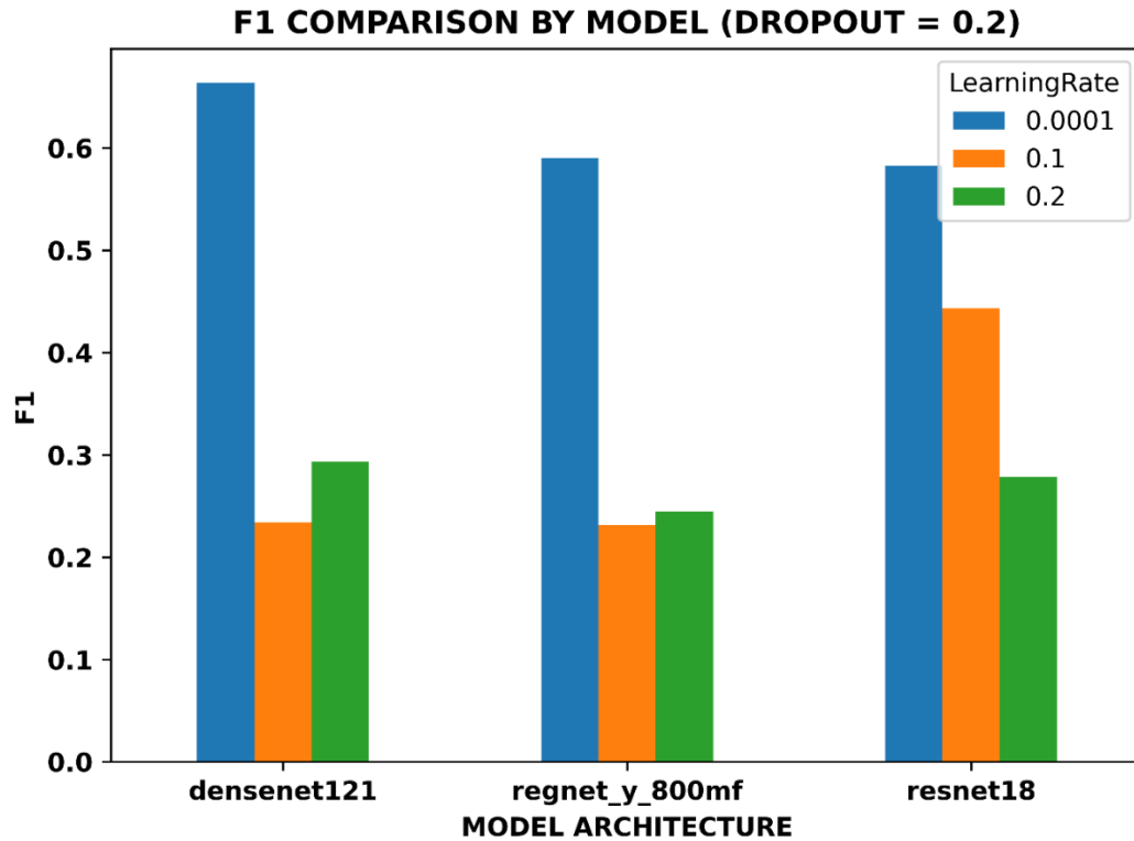
Figure 5 F1 COMPARISON BY MODEL (DROPOUT = 0.2)
