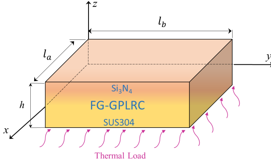
Figure 1. Graphical description of FG-GPLRC plate.
