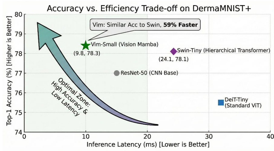
Figure 6. Accuracy and Efficiency Trade-off Analysis on the DermaMNIST+ Dataset.
