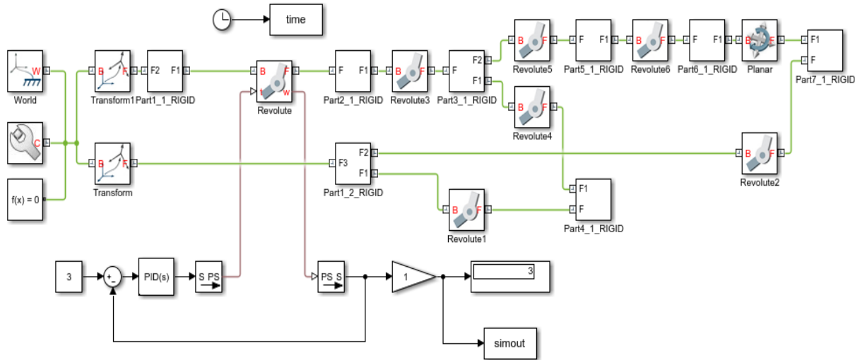
Figure 7. Block Diagrams of the Two-Loop Mechanism after PID Control is Applied
