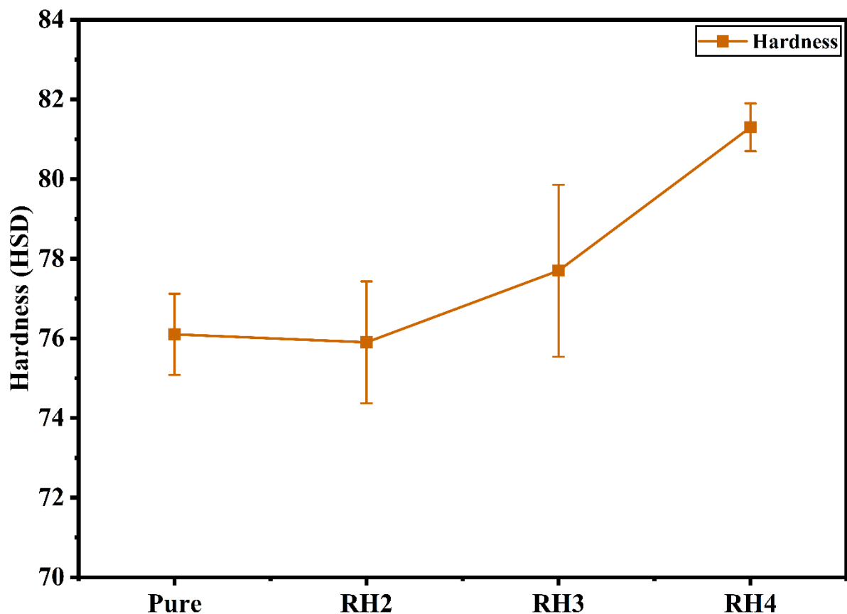
Figure 2. Shore D (HSD) hardness chart of reference and composite samples.
