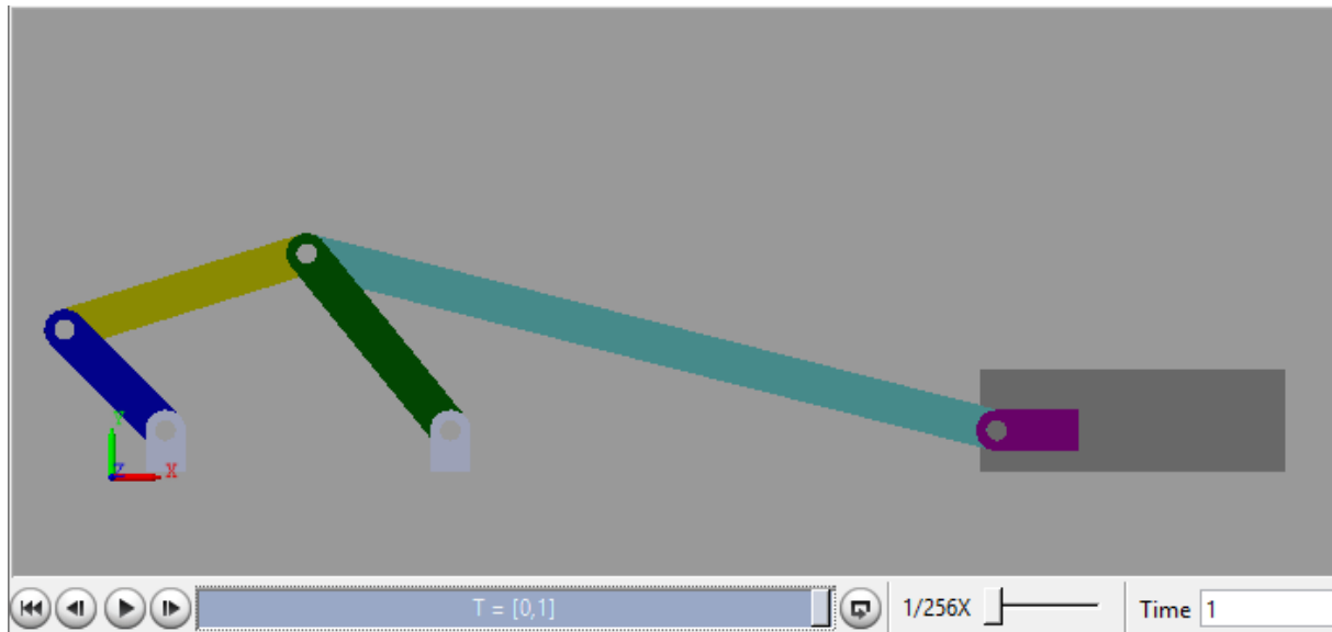
Figure 7. Two-Loop Mechanism Position in Matlab After PID Control
