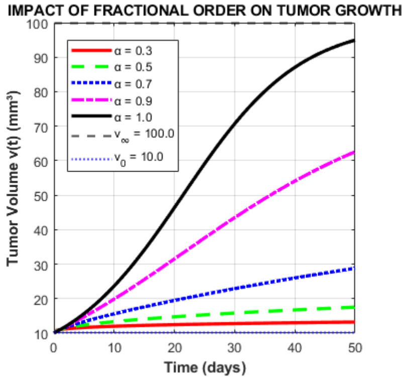
Figure 1. The growth of the tumor for various values of \alpha , where a = 1
