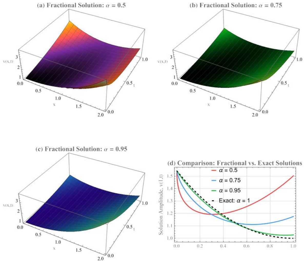
Figure 2. Analytical solutions v(x, t; \alpha) for the system of linear time-fractional differential equations.
