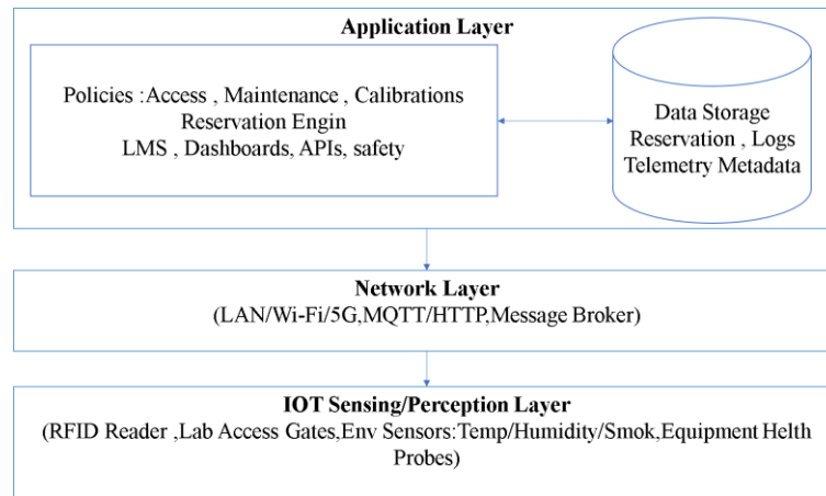
Fig 2: System Architecture
