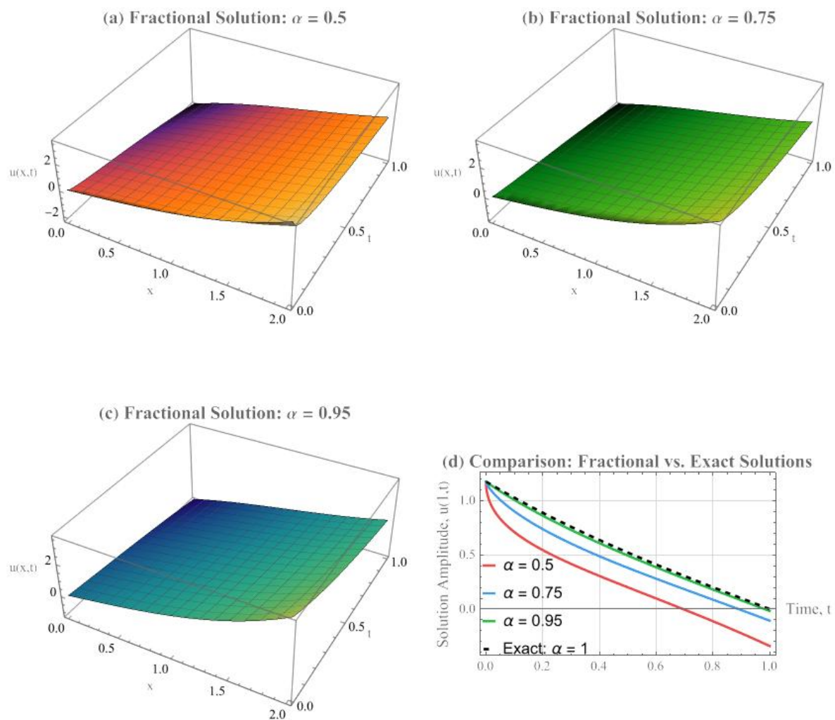
Figure 1. Analytical solutions u(x, t; \alpha) for the system of linear time-fractional differential equations.
