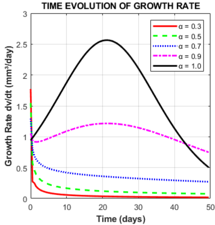
Figure 2. The growth rate of the tumor for various values of \alpha , where a = 1
