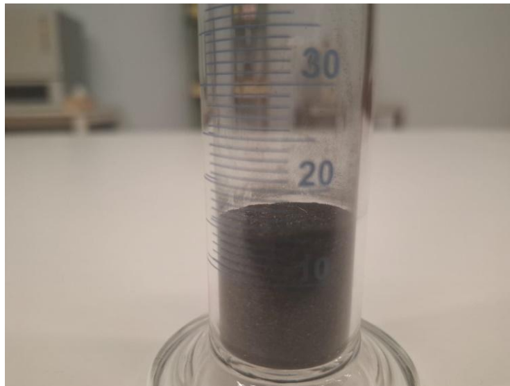
Figure 16. Measuring the volume occupied by the powder using a measuring cylinder.
