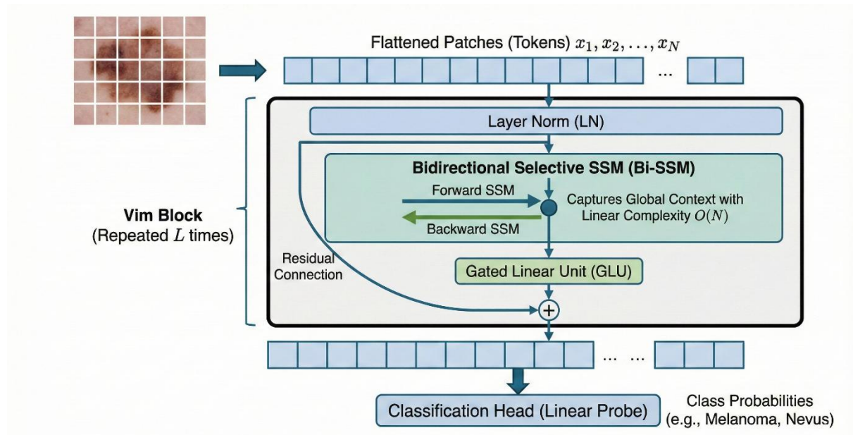
Figure 1. The Vision Mamba (Vim) Architecture 5
