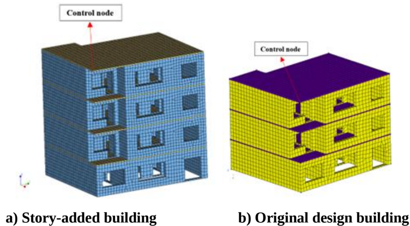
Figure 3. Finite element model of both buildings
