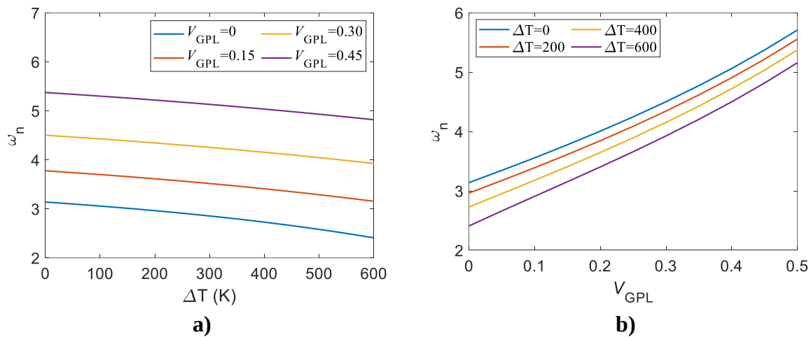
Figure 2. Examination of \omega_n with respect to V_{GPL} and \Delta T ( p=1, l_b/l_a=1 ).
