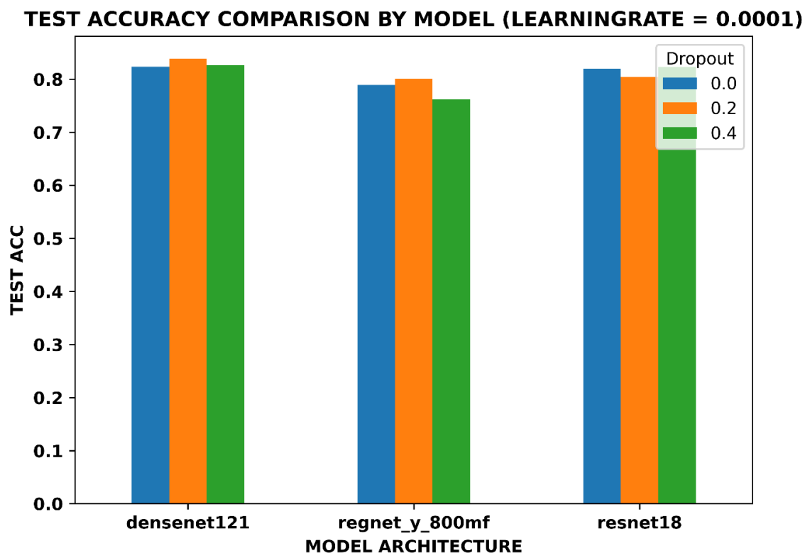
Figure 4 Test Accuracy Comparison by Model (Learning Rate = 0.0001)
