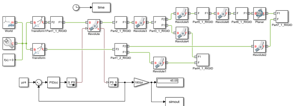
Figure 8. Block Diagrams of the Two-Loop Mechanism after PID Control is Applied
