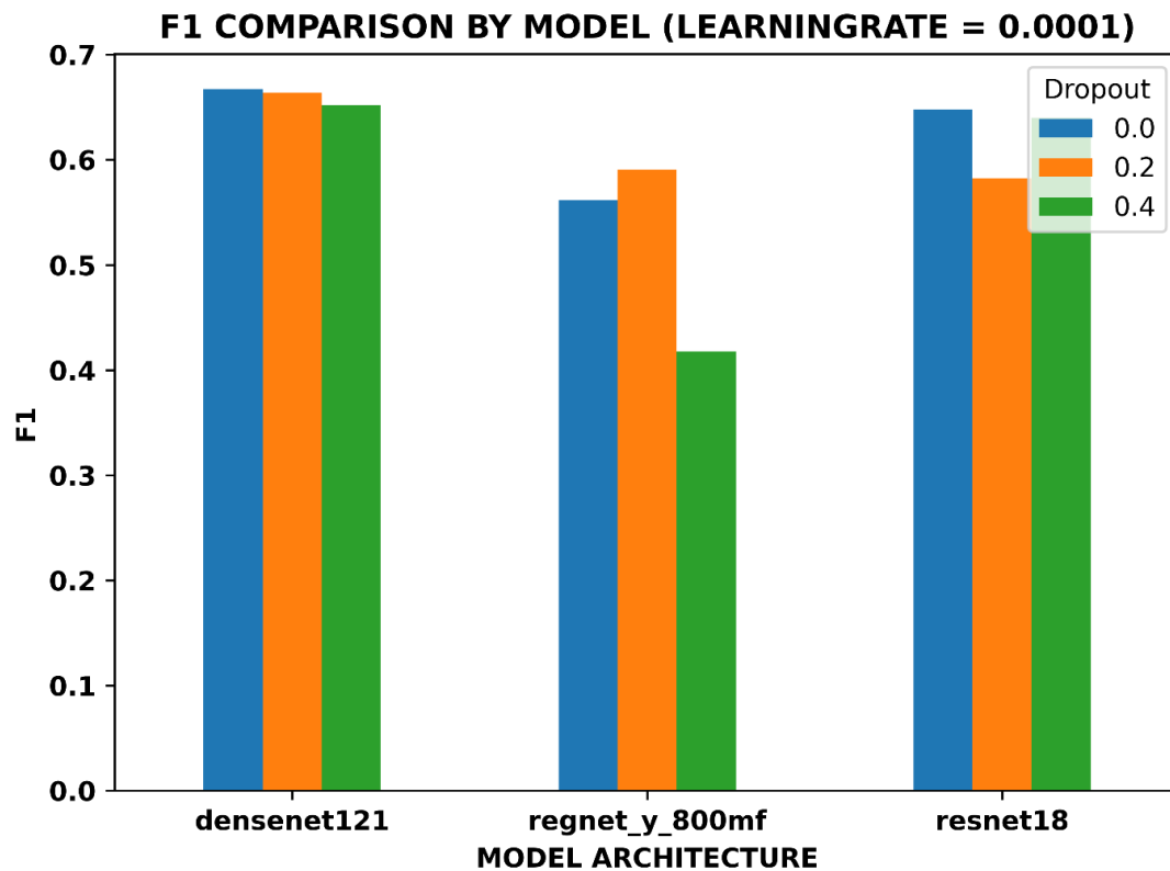
Figure 1 F1 Comparison by Model (Learning Rate = 0.0001)
