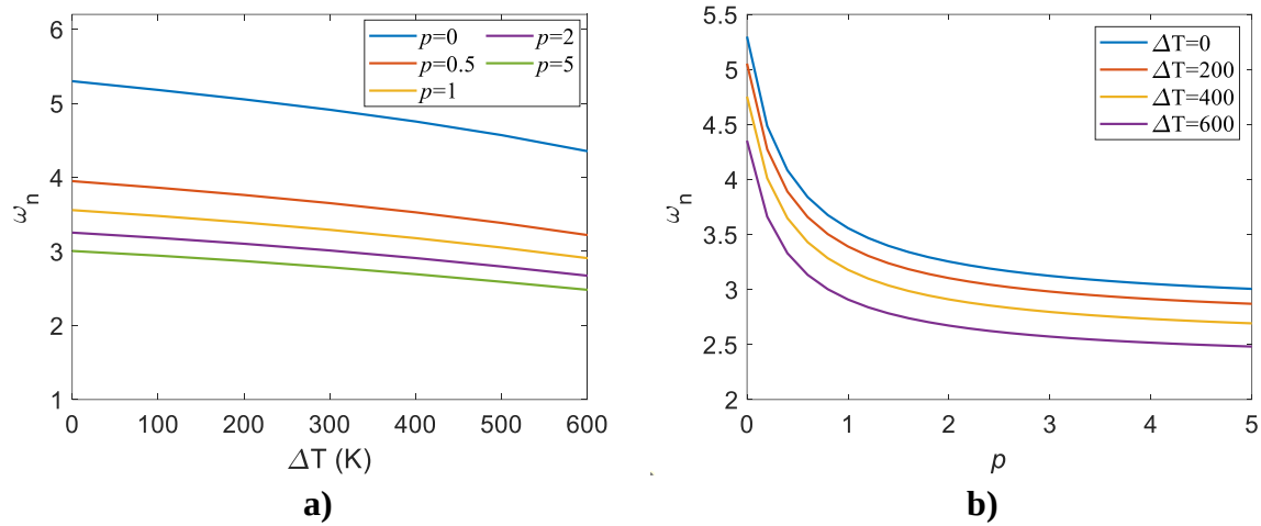
Figure 3. Examination of \omega_n with respect to p and \Delta T ( V_{\text{GPL}}=0.1 , l_b/l_a=1 ).
