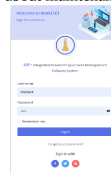
Fig 3: Login Page
