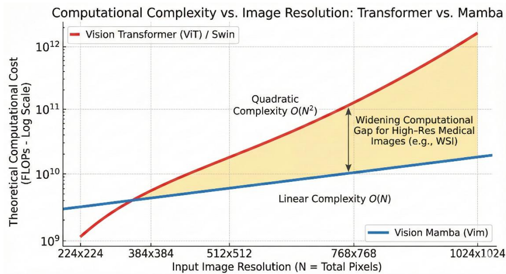
Figure 5. Theoretical Computation Complexity Analysis as a Function of Image Resolution (Logarithmic Scale).
