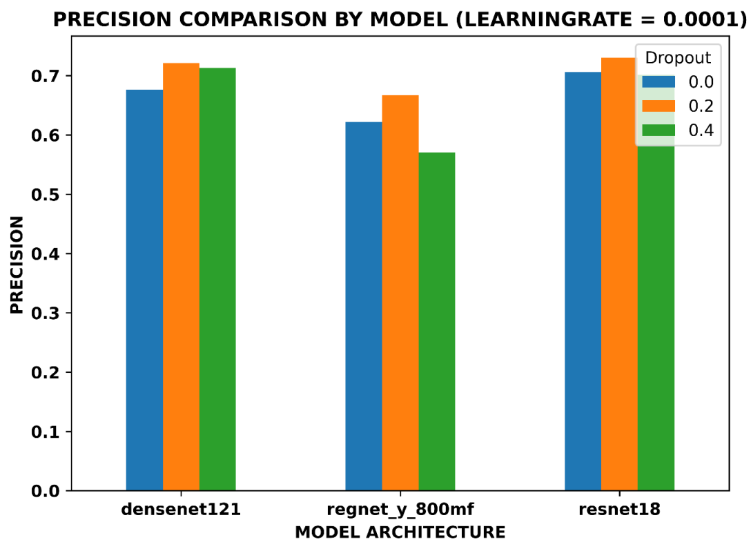
Figure 2 Precision Comparison by Model (Learning Rate = 0.0001)
