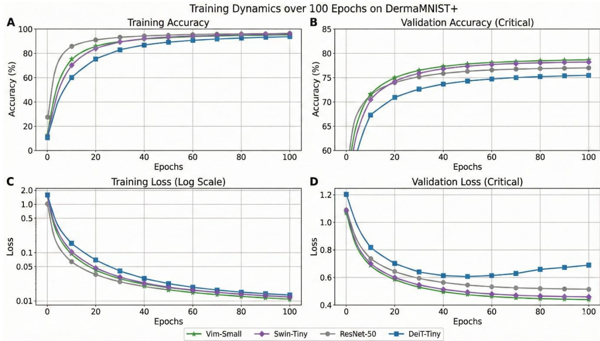
Figure 4. Training dynamics for all models
