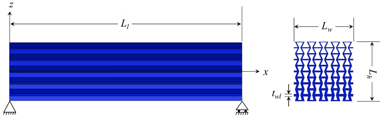
Figure 1. Re-entrant auxetic lattice beam model
