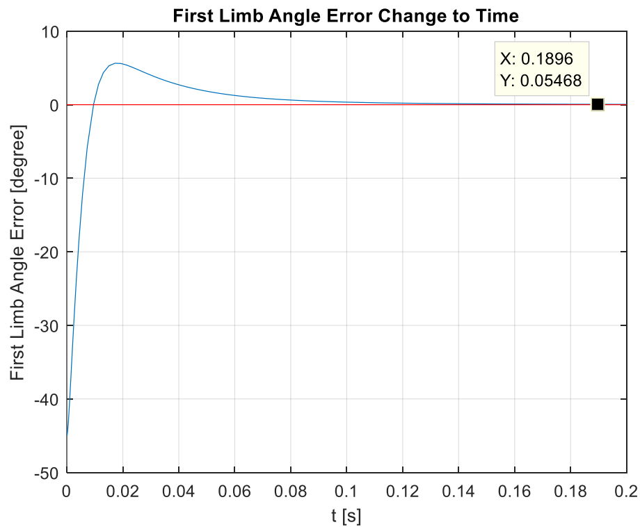
Figure 10. First Limb Angle Error Change to Time of Two-Loop Mechanism
