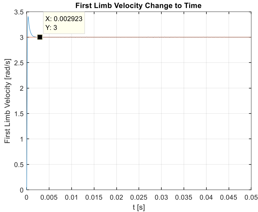
Figure 8. First Limb Angle Change to Time of Two-Loop Mechanism
