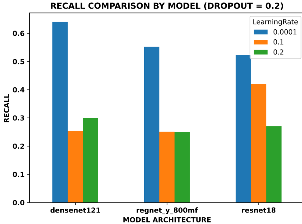
Figure 7 RECALL COMPARISON BY MODEL (DROPOUT = 0.2)
