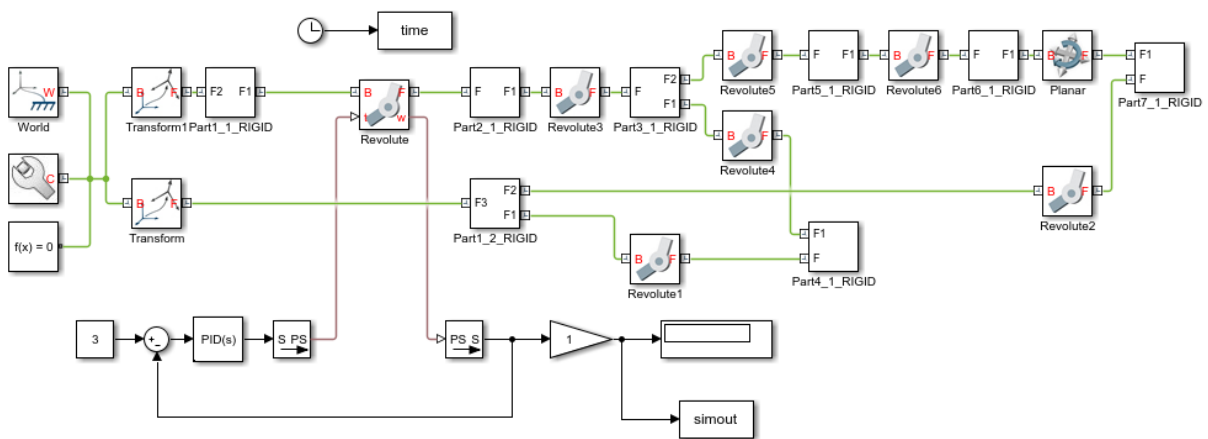
Figure 4. Block Diagram of Two-Loop Mechanism with PID
