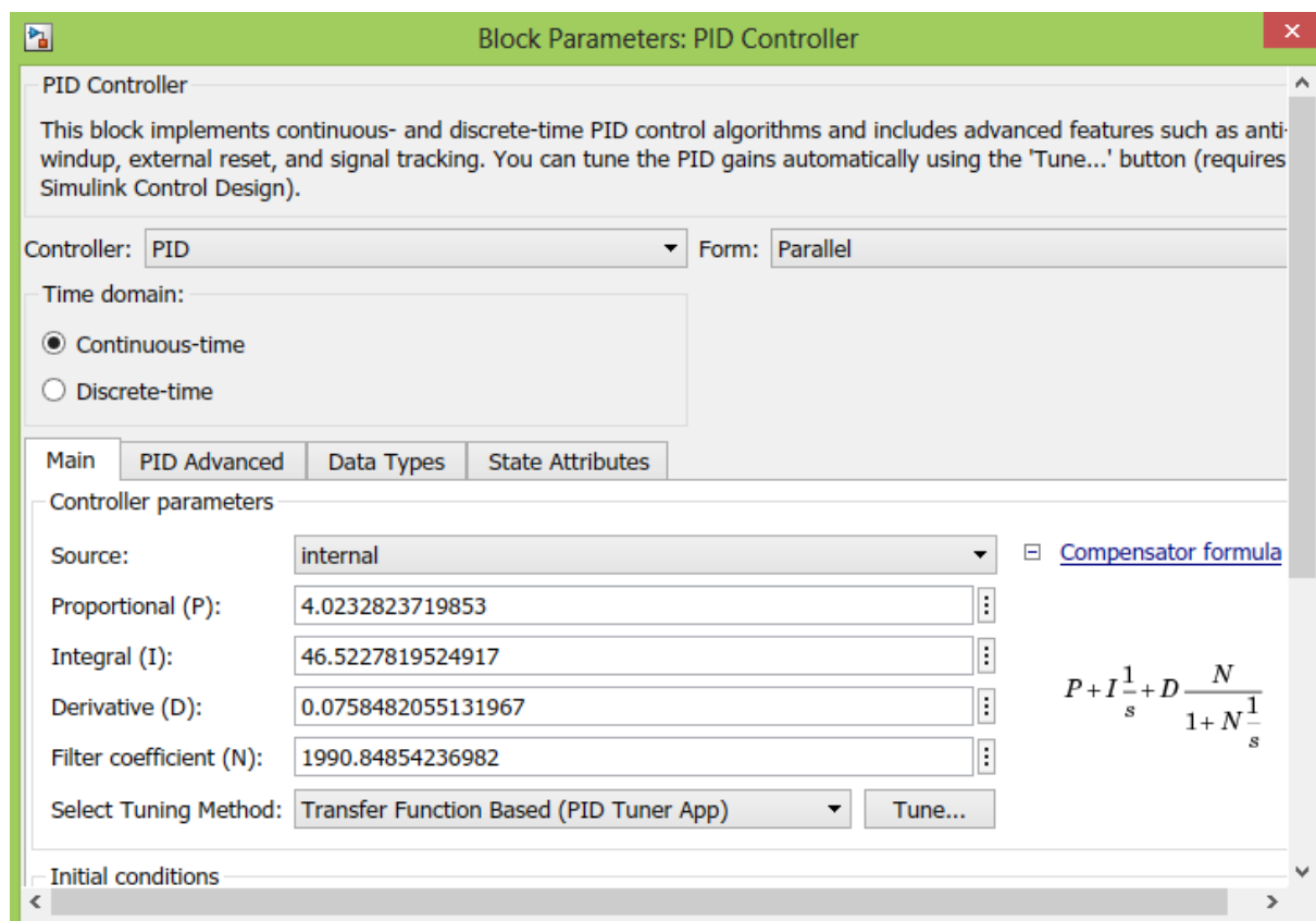
Figure 6. Display of the Mechanism's Gain Coefficients within the PID Block
