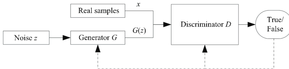
Fig.10. Computational procedure and architecture of a GAN. [7]
