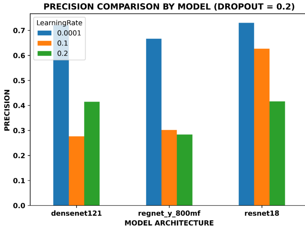
Figure 6 PRECISION COMPARISON BY MODEL (DROPOUT = 0.2)
