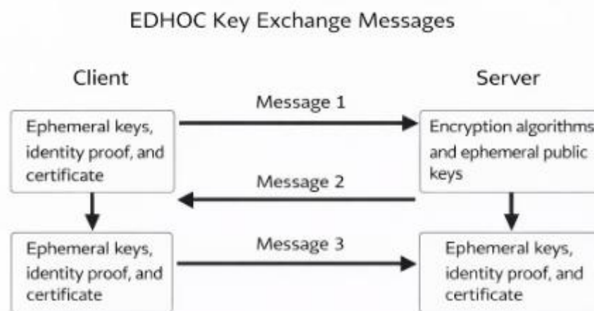
Figure 1. EDHOC Protocol Message Flow Diagram
