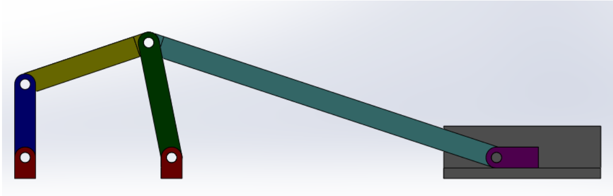
Figure 1. Solid Model of the Two-Loop Mechanism
