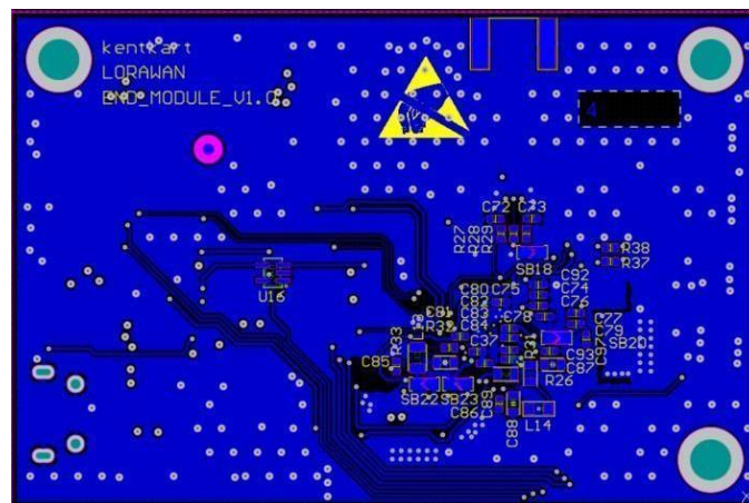
Figure 4. PCB Design Bottom Layer
