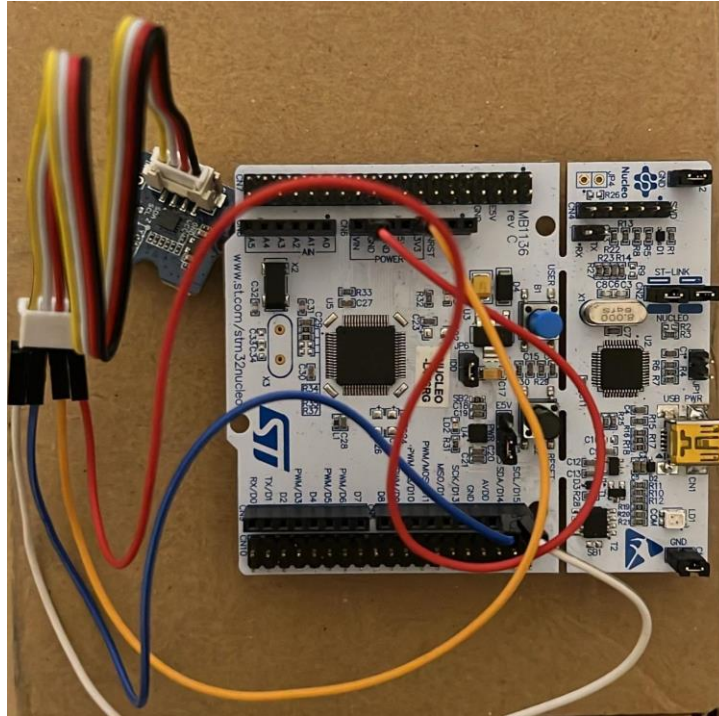
Figure 5: Setup
