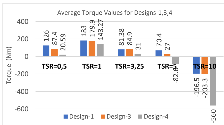
Figure 3.41. Average Torque Values for Designs-1,3,4
