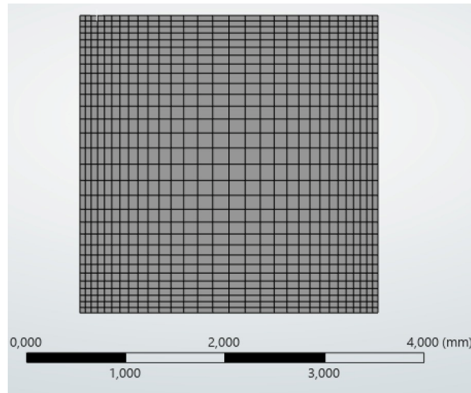
Figure 2. Grid distribution for square minichannel
